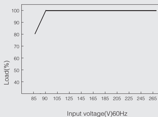
Static characteristic
