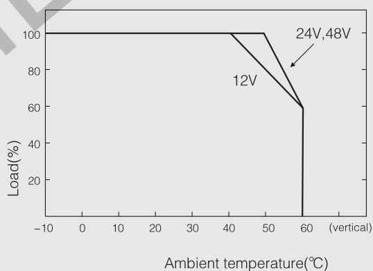
Derating curve
