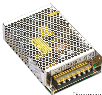
Dimension: 159 × 97 × 38mm
